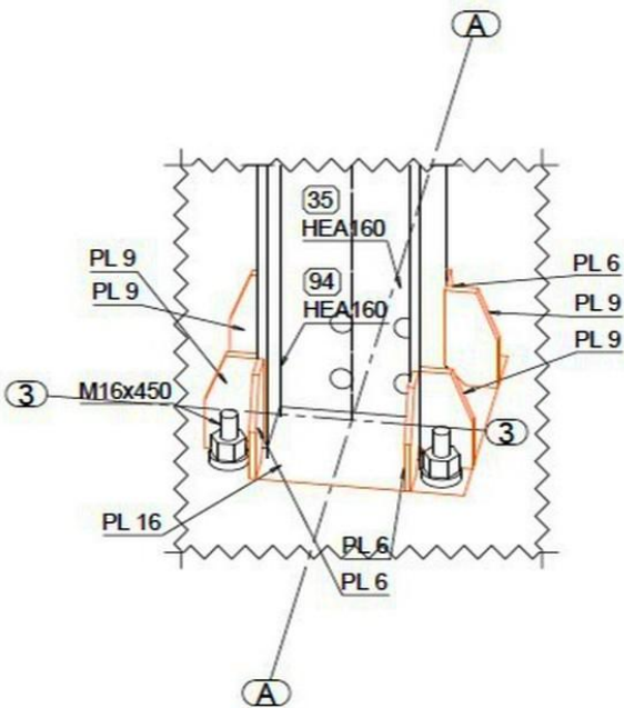
D Detalle Platina Base Columna HEA160 001 1:5
